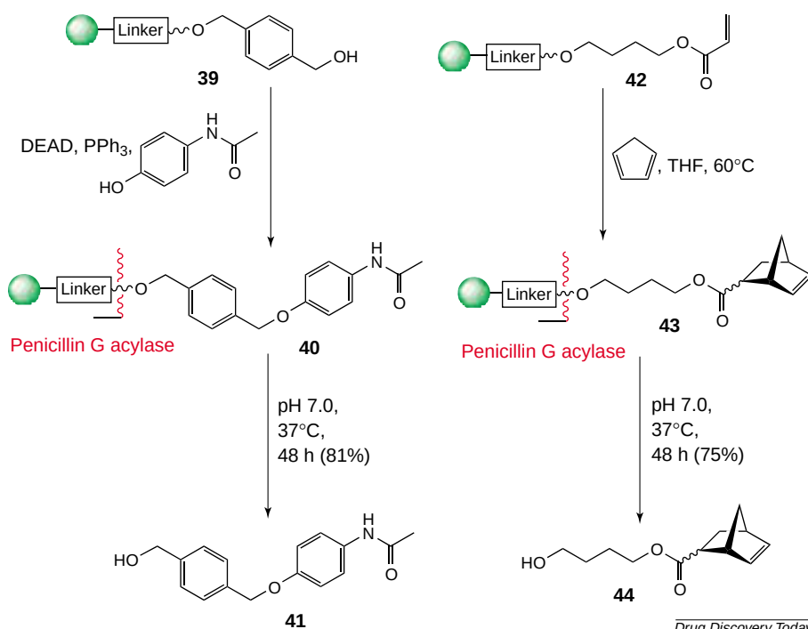
Figure 11. Mitsunobu and Diels–Alder reaction on enzyme-labile linker conjugates.
