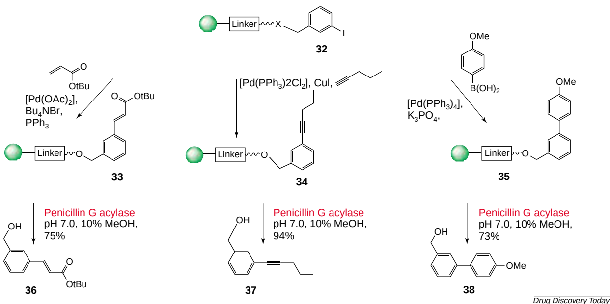
Figure 10. Pd(0)-catalyzed reactions on enzyme-labile linker conjugates.
